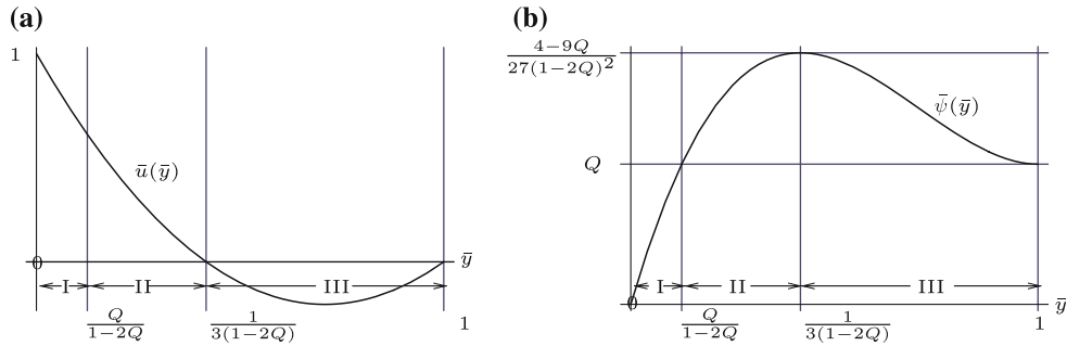
Fig. 4 An illustration of the flow speed \bar{u} in the case 0 < Q < 1/3 from (10) and stream function from (14) with regions I, II and III marked accordingly. (a) Velocity profile and (b) stream function
