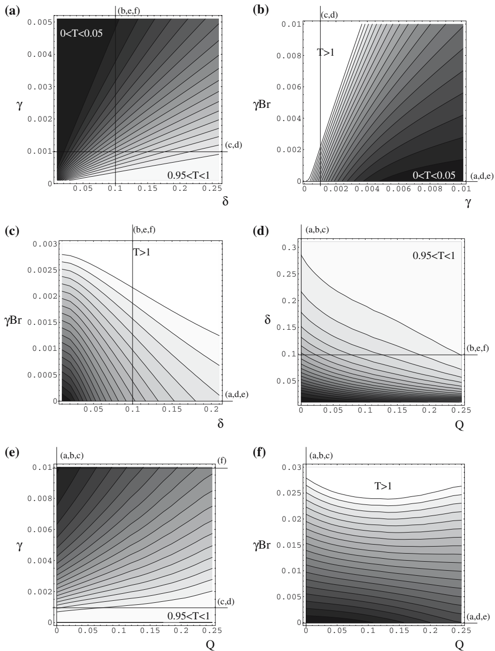
Fig. 10 Parametric plots of maximum temperature T_0 at the exchanger outlet z = 1 predicted by averaged model. The temperature contours are at intervals of 0.05 and the black regions are defined by 0 < T_0 < 0.05 . Dotted lines indicate projections of other graphs contained in this figure on the plane of each graph. (a) Q = 0 , Br = 0 , (b) Q = 0 , \delta = 10^{-1} , (c) Q = 0 , \gamma = 10^{-3} , (d) Br = 0 , \gamma = 10^{-3} , (e) Br = 0 , \delta = 10^{-1} and (f) \gamma = 10^{-2} , \delta = 10^{-1}
